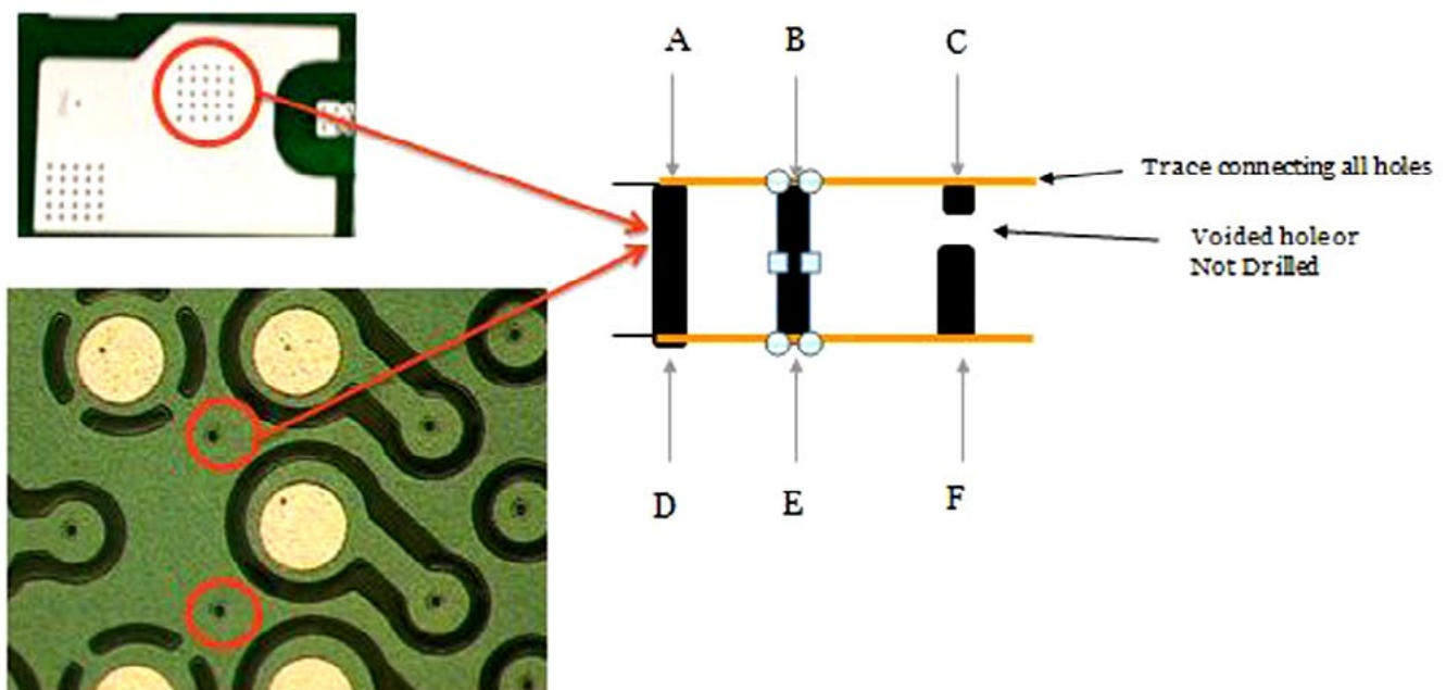
Figure 5: Voids in circular nets.
