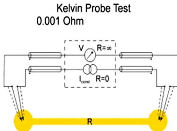
Figure 3: A typical Kelvin circuit.
